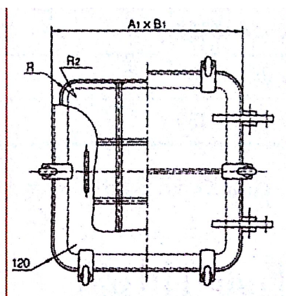
CB* 3274-85 通气舱口盖 Breather Hatch Cover
