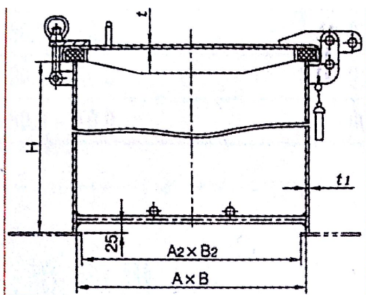
CB* 3274-85 通气舱口盖 Breather Hatch Cover
