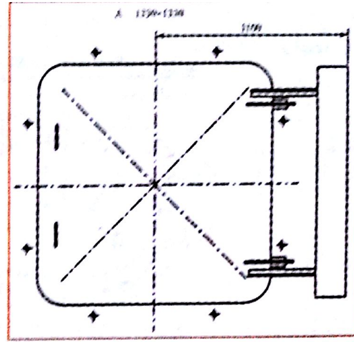
GB/T 3728-1995 舱口盖 Hatch Cover (Type B)
